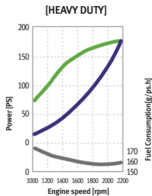
Performance Curve
