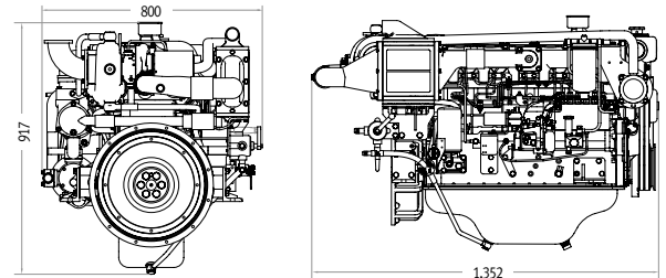
Engine Dimension
